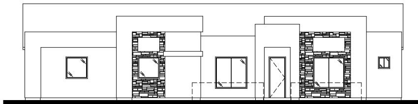
FRONT ELEVATION 'C'
